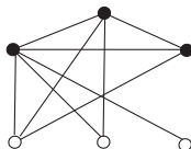
FIG. 3.2. The 3rd half-graph H_3
