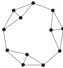
FIG. 2.1. The necklace N_3
