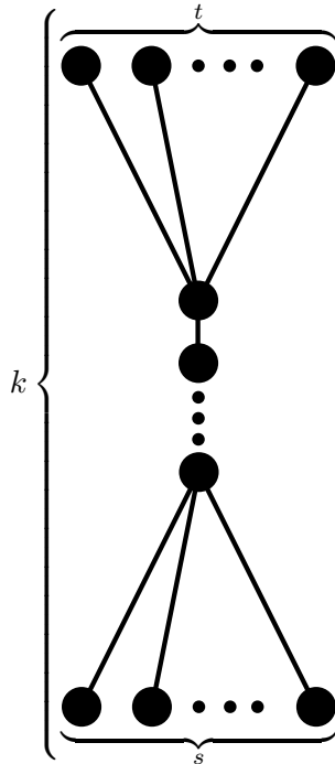
Figure 1.8 The broom \mathcal{P}_k(s, t) .
