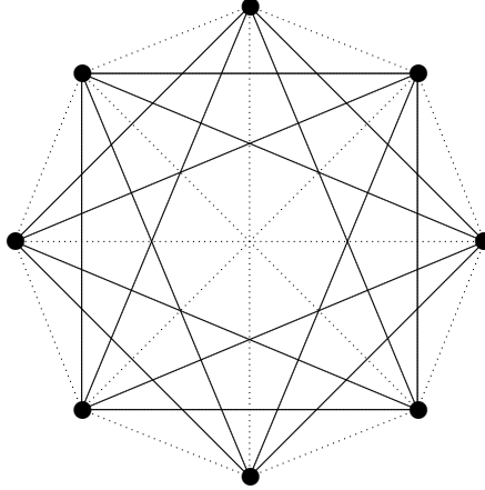
FIGURE 8. A square representation of 6_7
