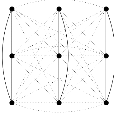
FIGURE 6. Unique minimal square representation of 4_7
