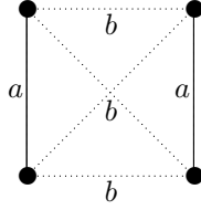
FIGURE 3. Unique minimal square representation of 1_7
