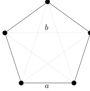
FIGURE 7. Unique square representation of 5_7
