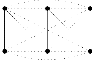
FIGURE 5. Unique minimal square representation of 3_7
