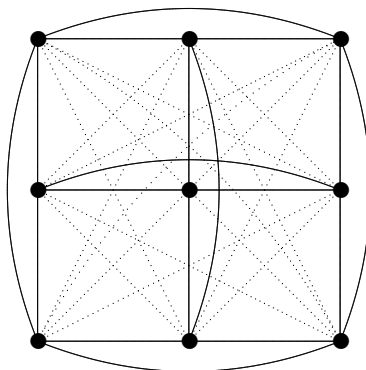
FIGURE 9. A square representation of 7_7
