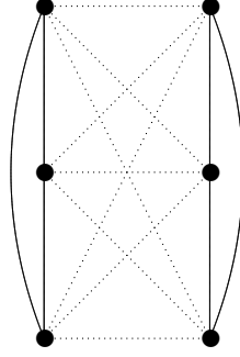
FIGURE 4. Unique minimal square representation of 2_7
