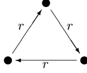
FIGURE 2. Unique square representation of 2_3
