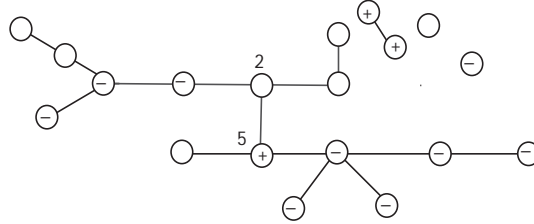
FIG. 5.2. The signed forest \mathcal{G}(Z) - Q_1 resulting from the first iteration of Algorithm 5.4
