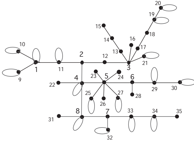
FIG. 5.6. The tree T = T_1
