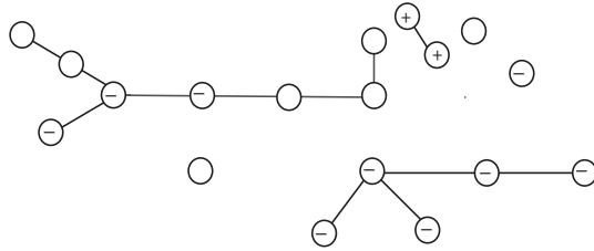
FIG. 5.3. The signed forest \mathcal{G}(Z) - Q
