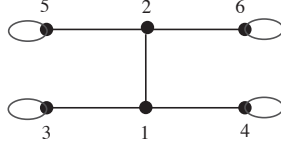
FIG. 4.1. The double path T_{DP}
