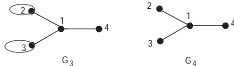
FIG. 2.1. Graph G_3 that requires nonsingularity and graph G_4 that requires singularity
