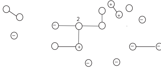
FIG. 5.4. The signed forest \mathcal{G}(Z) - Q_1
