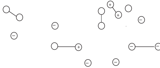
FIG. 5.5. The signed forest \mathcal{G}(Z) - Q
