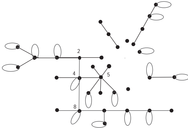
FIG. 5.7. The forest T - Q_1 resulting from the first iteration of Algorithm 5.4
