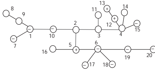
FIG. 5.1. The signed tree \mathcal{G}(Z)
