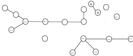
FIG. 2.3. The signed forest \widehat{\mathcal{G}}(Z) - Q
