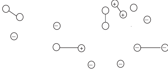
FIG. 2.5. The signed forest \widehat{G}(Z) - Q
