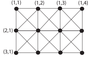
Figure 17: The 3 \times 4 strong product.
