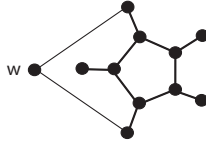
Figure 2: The graph G for Example 2.5
