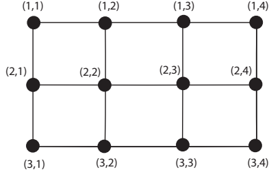
Figure 9: The 3 \times 4 grid graph P_3 \square P_4 .
