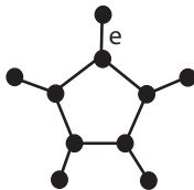
Figure 5: The pentasun H_5 for Example 2.18
