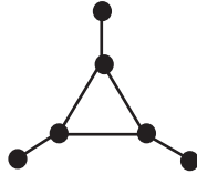
Figure 4: The graph H_3 in Example 2.11
