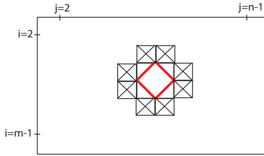
Figure 19: Covering of king grid for zero spread -1 .
