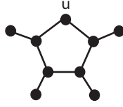
Figure 3: A counterexample to the converse of Theorem 2.8
