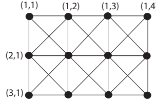
Figure 17: The 3 \times 4 strong product.
