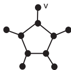
Figure 1: The pentasun H_5
