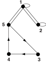
FIG. 4.4. Forced digraph \Gamma(Z) for G_{5,3}
