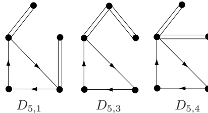
FIG. 4.2. Forced placement of non-loop arcs
