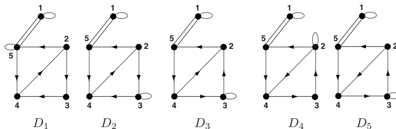
FIG. 4.9. Possible digraphs for G_{6,5}
