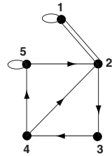
FIG. 4.7. Forced digraph \Gamma(Z) for G_{6,2}
