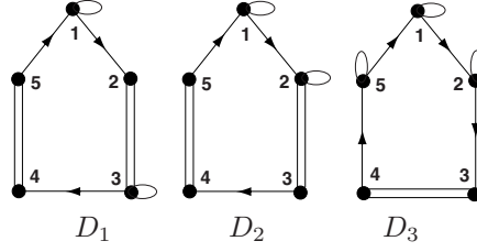
FIG. 4.5. Possible digraphs \Gamma(Z) for G_{5,5}
