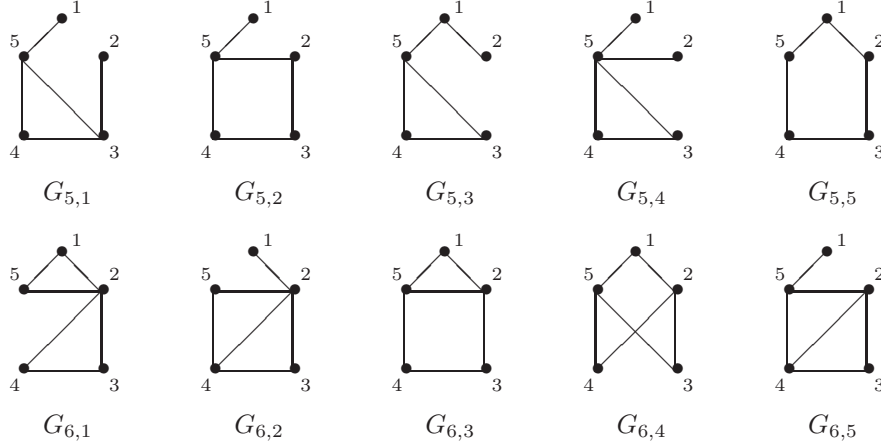
FIG. 4.1. Connected Order 5 graphs with 5 or 6 edges
