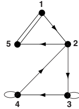
FIG. 4.6. Forced digraph \Gamma(Z) for G_{6,1}
