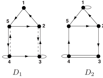
FIG. 4.8. Possible digraphs for G_{6,3}
