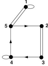
FIG. 4.3. Forced digraph \Gamma(Z) for G_{5,2}
