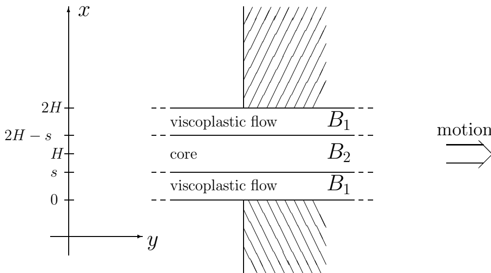
FIG. 1. Geometrical Configuration
