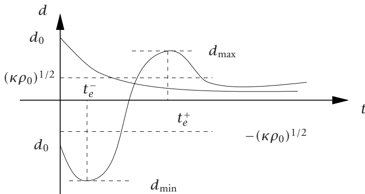
Figure 5: d_0^2/2\rho_0 < k < d_0^2/\rho_0
