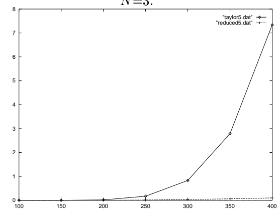
Figure 7: The relative error with increasing R . The approximation order varies from N=0 to 5. Taylor method is solid, reduced basis dashed.
