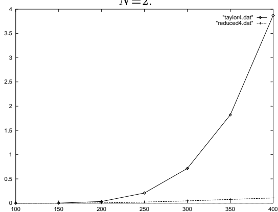
Figure 7: The relative error with increasing R . The approximation order varies from N=0 to 5. Taylor method is solid, reduced basis dashed.
