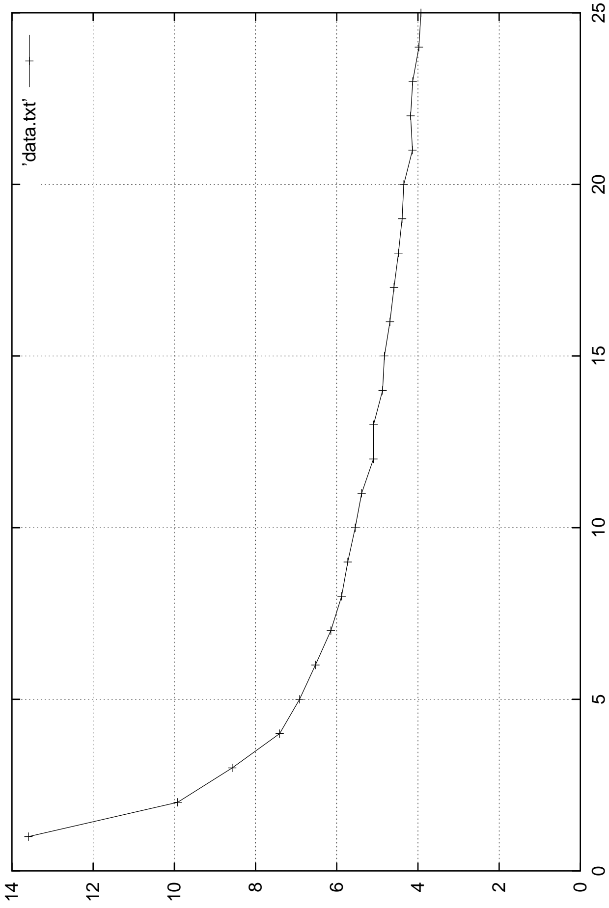
Number of Clusters vs Total Energy, Normalized Data
